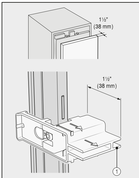
Cabinet-front thickness of 1\frac{1}{2} " (38 mm)
