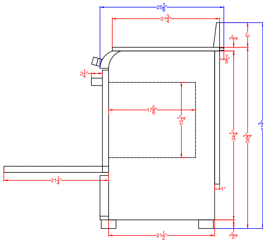
PROFILE VIEW
