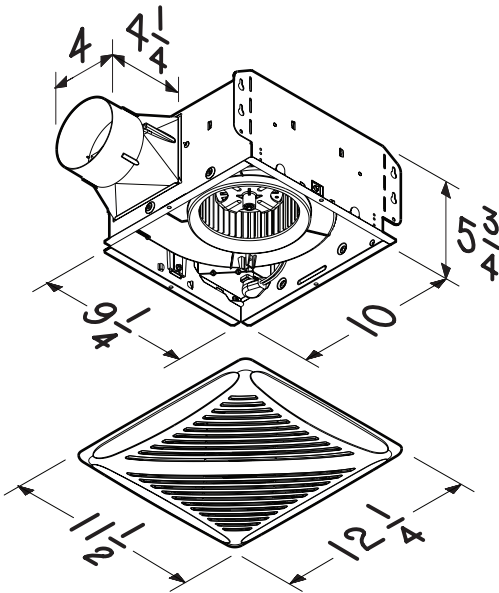
Dimensions shown are in inches.
