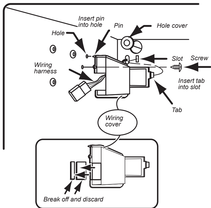
Ice maker wiring cover
