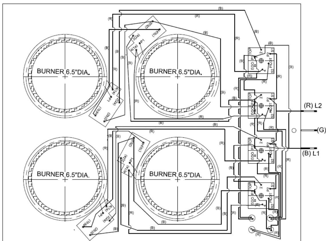
Wiring Diagram
