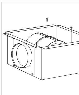
Internal blower installation
