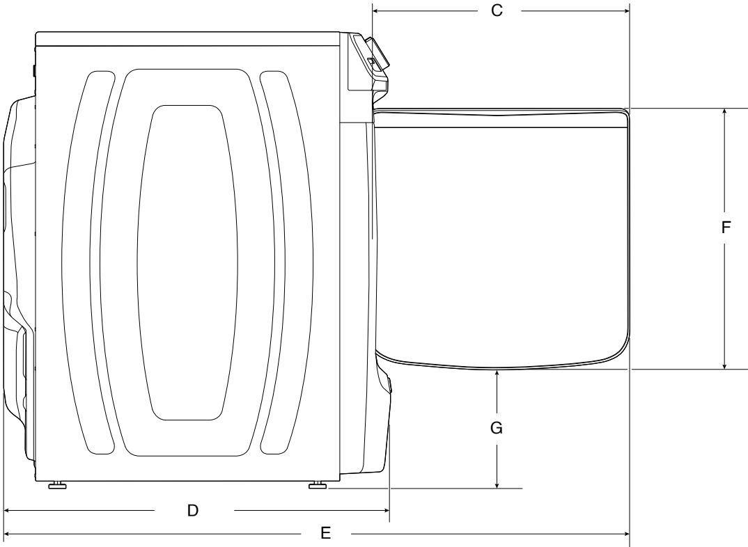
SIDE VIEW
