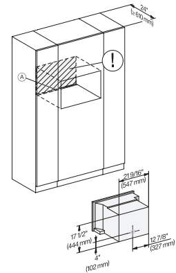
CVA7370, installation drawing, installation, 30 Inch, Proud A – Cut-out (1 1/2" x 20" / 38 mm x 508 mm) in the bottom of the cabinet for power cord and ventilation, – Electrical and water supplies are recommended to be placed in adjacent cabinetry., Additional cabinet depth is required when placing the electrical and water supplies behind the appliance., E = Electric connection
