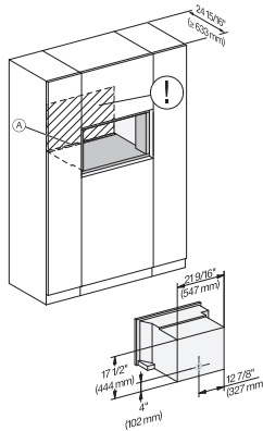
CVA7370, installation drawing, installation, 30 Inch, Flush inset
