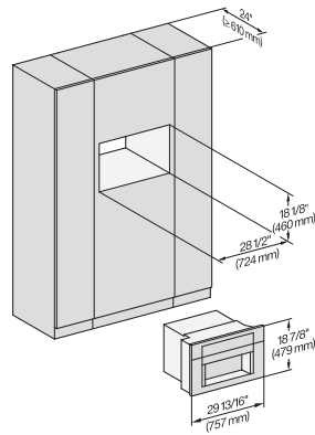
CVA7370, CVA7775, installation drawing, built in, 30 Inch, Proud
