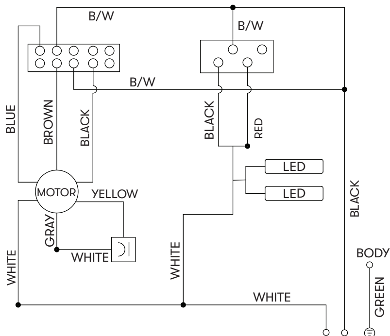
AK1100Bx, AK1136Bx Wiring Diagram
