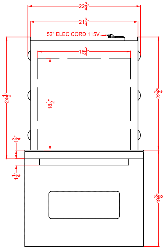
TOP VIEW
