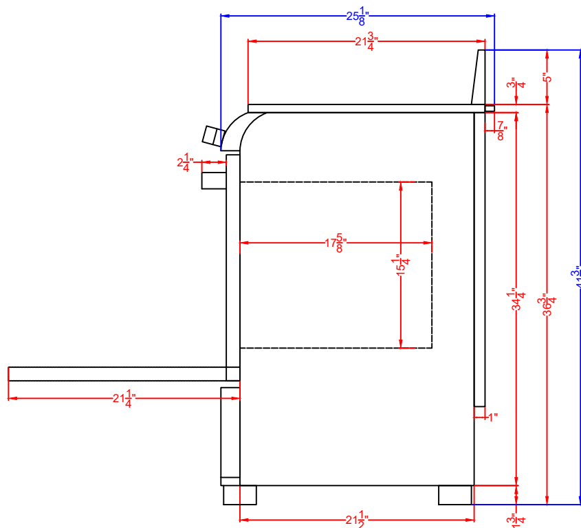
PROFILE VIEW
