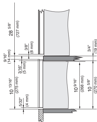
ESW 6*80, CLST (detailed installation drawing) – USA
