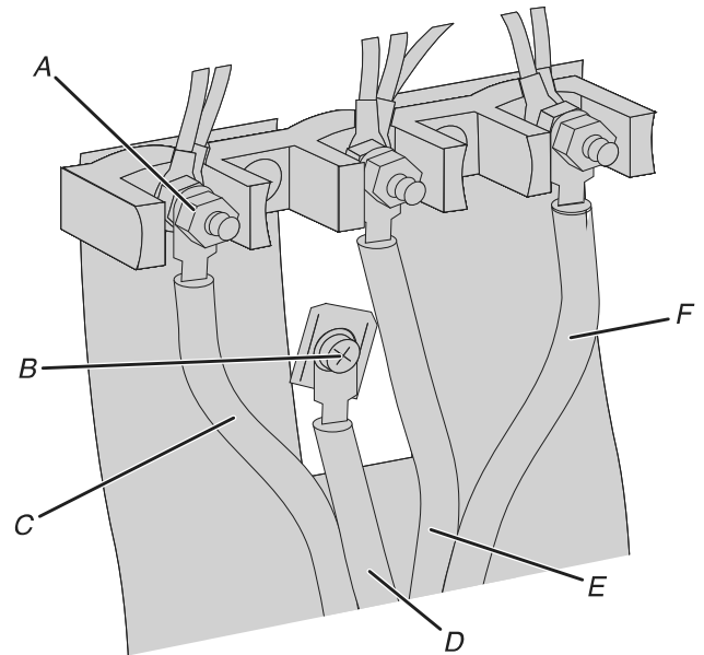
A. 10-32 hex nut B. Ground-link screw C. Line 2 (red) D. Green ground wire E. Neutral (center) wire F. Line 1 (black)
