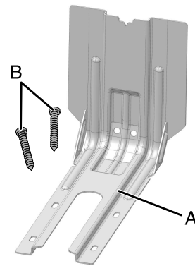
A. Anti-tip bracket B. #12 x 1½" (41 mm) screws (2)
