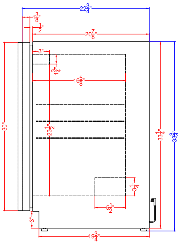
Profile View
