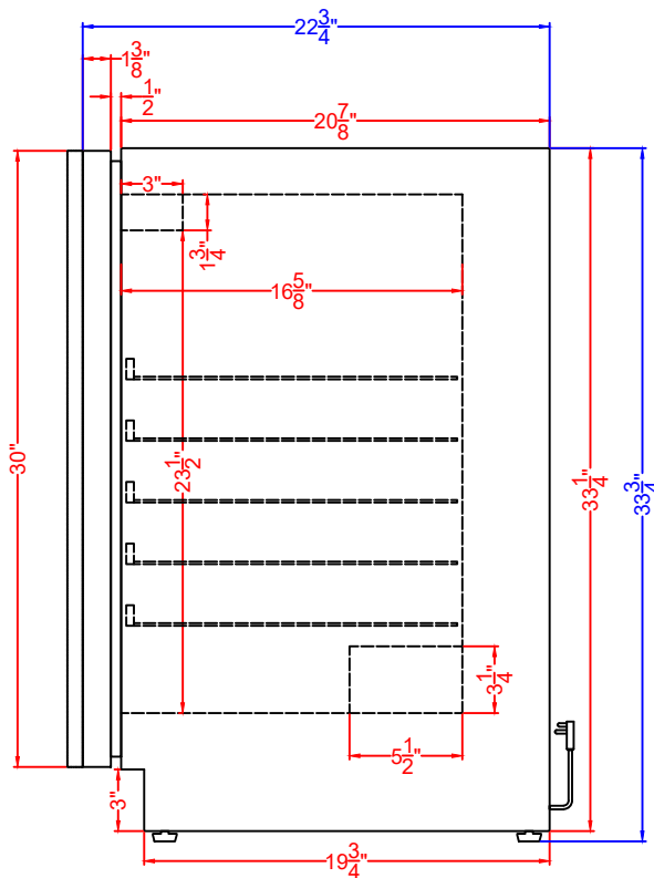
Profile View
