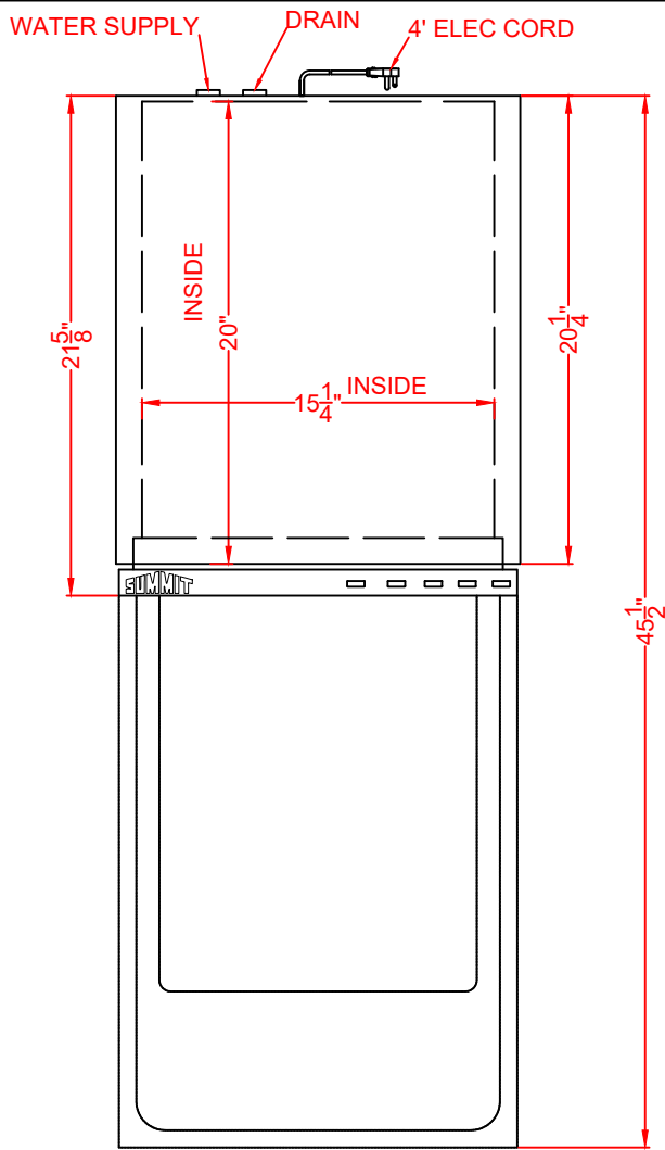
TOP VIEW
