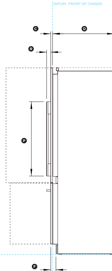
PROFILE VIEW
