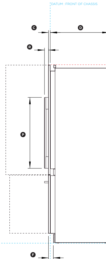
PROFILE VIEW
