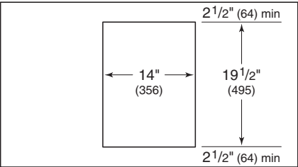
COUNTERTOP CUT-OUT
