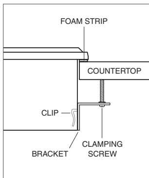
Module installation.
