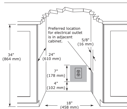
Cabinet Cut-Out
