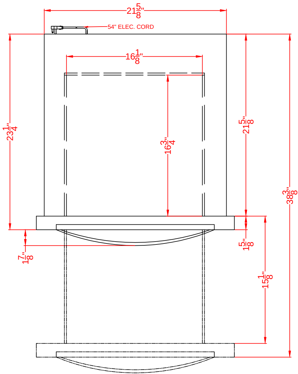
TOP VIEW
