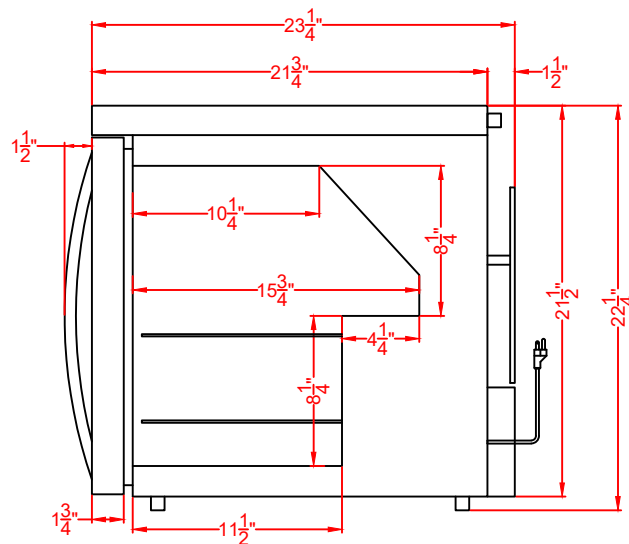
PROFILE VIEW
