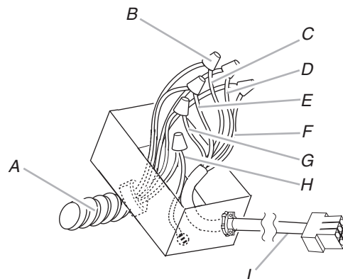
A. UL Listed or CSA approved 1/2" (13 mm) wiring conduit B. UL Listed wire connectors C. Black wires D. White wires E. Red wires F. Blue wires G. Gray wires H. Green (or yellow/green) and green/yellow wires I. Motor electrical plug cable operating.
