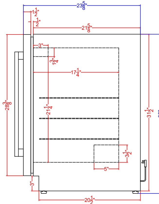
Profile View
