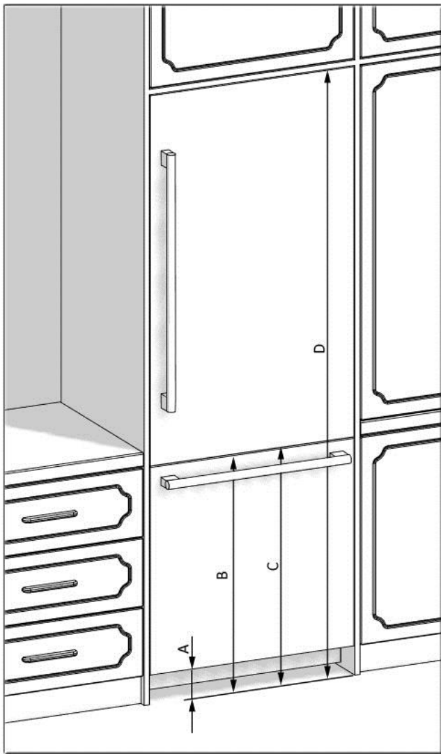
Height of the Kitchen Countertop Based on the Min./Max. Height of the Cabin;
