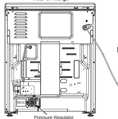
Pressure Regulator
