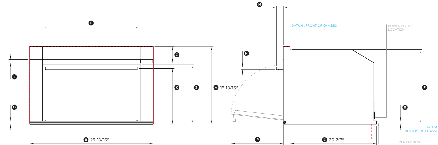
FRONT VIEW
