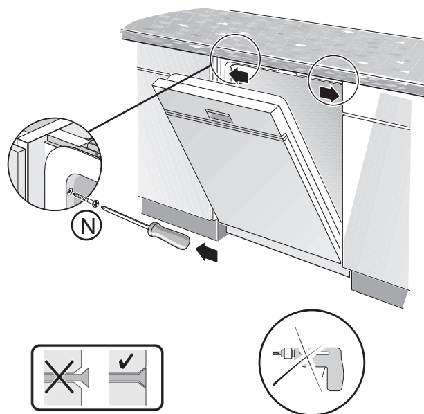
Figure 22 For Alternate Side Mount
